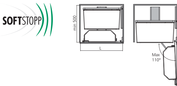
➤ Armoire coulissante TANDEM
